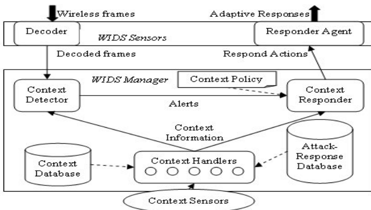
Fig. 1. CAWAnalyser Architecture
