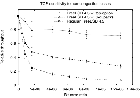
Fig. 7. Relative performance (1 Mbps, 50 ms)
