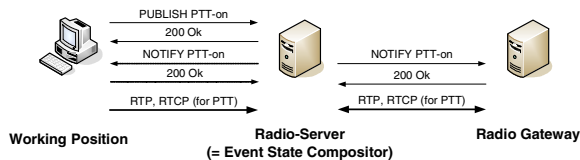
Fig. 2. Request and Grant of Radio Access
