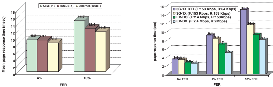
Fig. 5. Web page response time for different RAN transport and 3G technology
