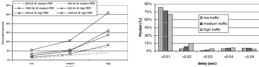
Fig. 3. left: Discarded packets (GBN algorithm) - right: Resequencing delay (SRPB algorithm)
