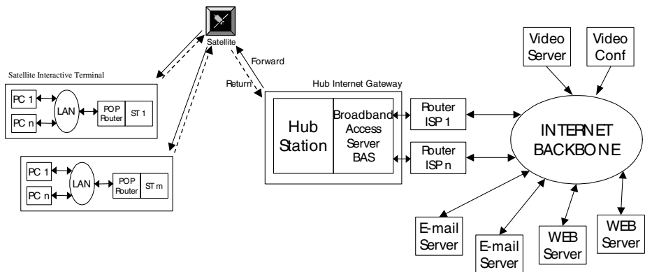
Fig. 1. TRANSAT System Architecture
