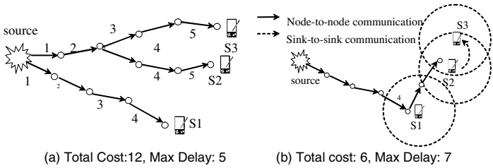
Fig. 4. Two approaches of data dissemination to multiple sinks
