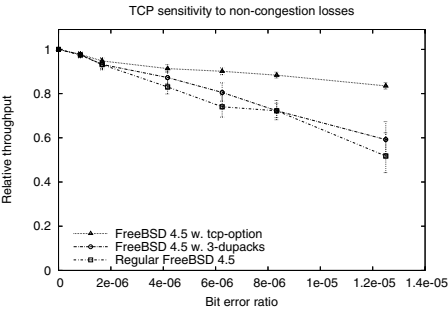
Fig. 11. Relative performance (40 kbps, 50 ms)
