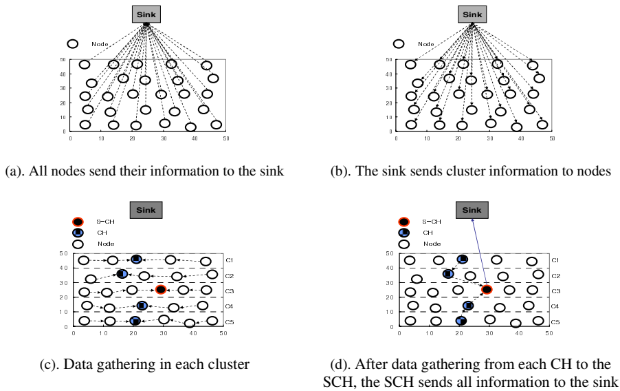
Fig. 1. Multi-hop routing through Super Cluster Header
