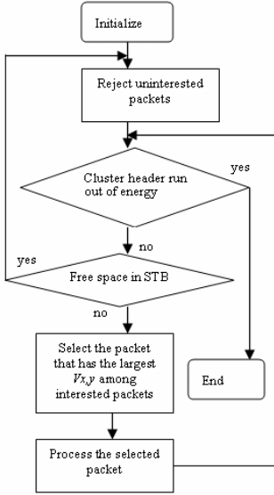
Fig. 2. Flowchart and source code of ETRI-PS
