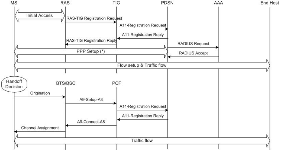
Fig. 3. Signaling and data flows
