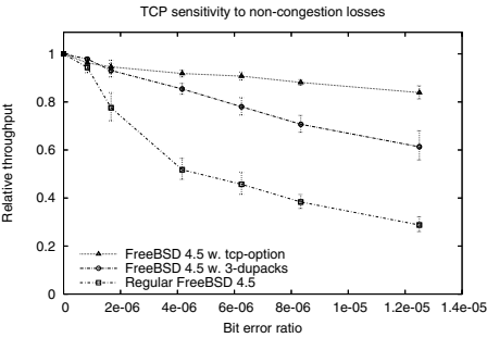
Fig. 9. Relative performance (160 kbps, 50 ms)
