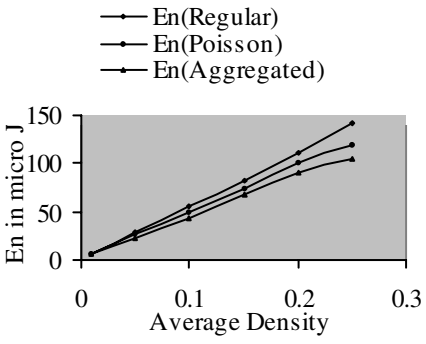
Fig. 4. En vs. Average Density
