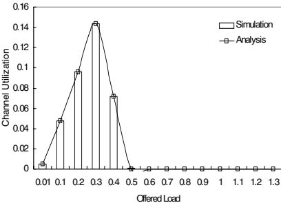
(f) Channel utilization of BE flows (analytical and simulation results)
