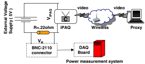
Fig. 9. Setup for our measurements
