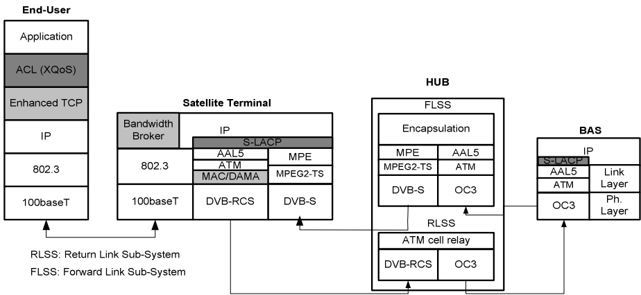
Fig. 2. TRANSAT Protocol Stack
