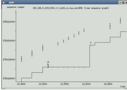
Fig. 4. With 3-dupacks loss notification
