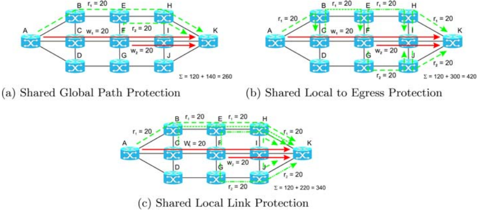
Fig. 1. Example of a path configuration for shared global path protection, shared local link protection and shared local to egress protection. The capacity requirements (working+protection) of the example configurations are shown in each figure
