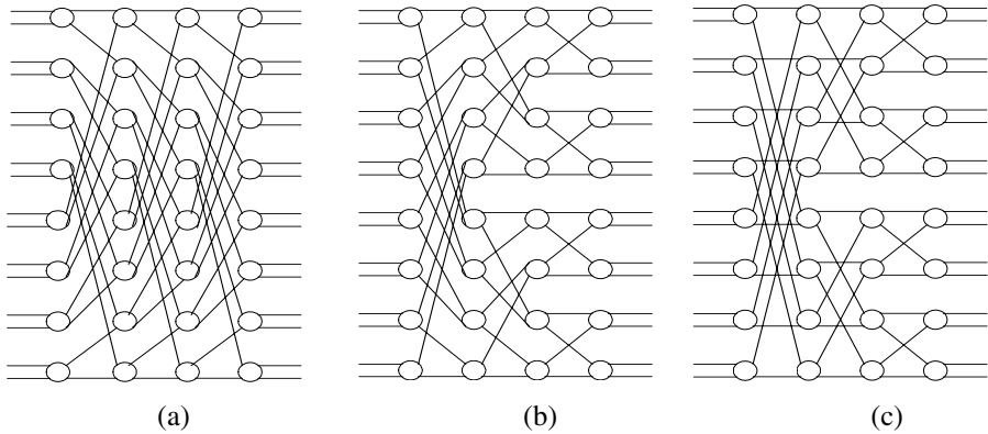
Fig. 1. Conventional layouts for (a) Shuffle (b) Baseline (c) Banyan networks
