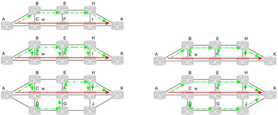
Fig. 2. Resilience resources comparison configuration. Left: Shared local link protection requires more capacity than shared global path protection. Right: Shared local to egress protection requires maximum the capacity of shared local link protection, however, more than shared global path protection
