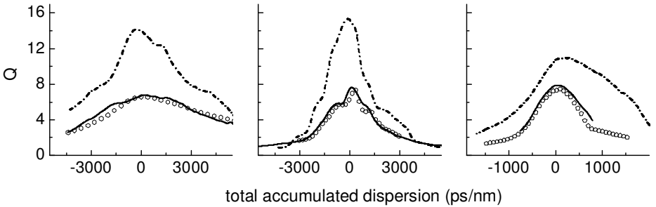
Fig. 2. Q-factor of the channel at 193.4 \text{ THz} versus total accumulated dispersion for NRZ-DQPSK (left), NRZ-DPSK (middle) and NRZ modulation (right) for full inline dispersion compensation. SPM only (dashed), multi channel SSF calculations (solid) and semi-analytic model (symbols)
