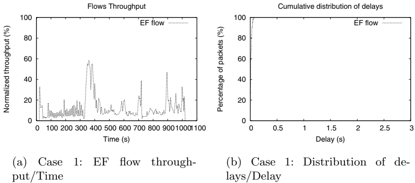
Fig. 3. Throughput and delays curves in the first case
