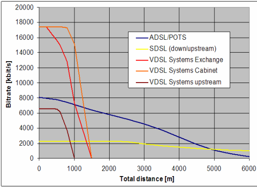
Fig. 5. Trade-off between bit-rate and range for ADSL, SDSL, and VDSL
