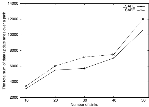
Fig. 5. The sum of all nodes’ update rates over a dissemination path
